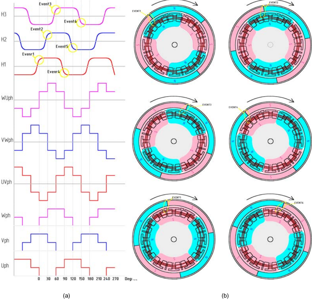
Figure 2. BLDC Coil Phase Voltage Switching (a) and Rotor Rotation Phases (b)
