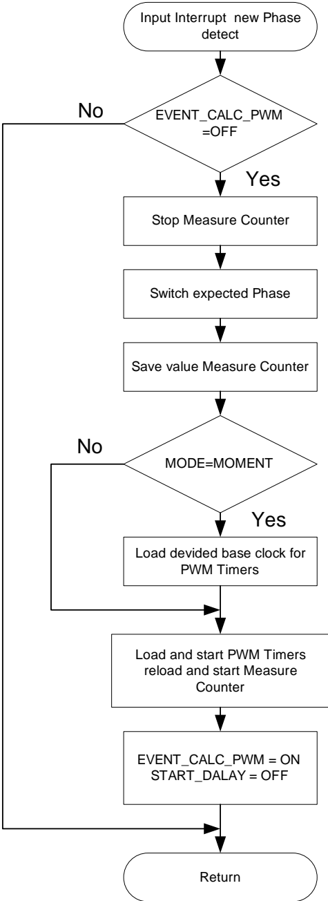
Figure 8. Sensor Comparator Interrupt Flowchart
