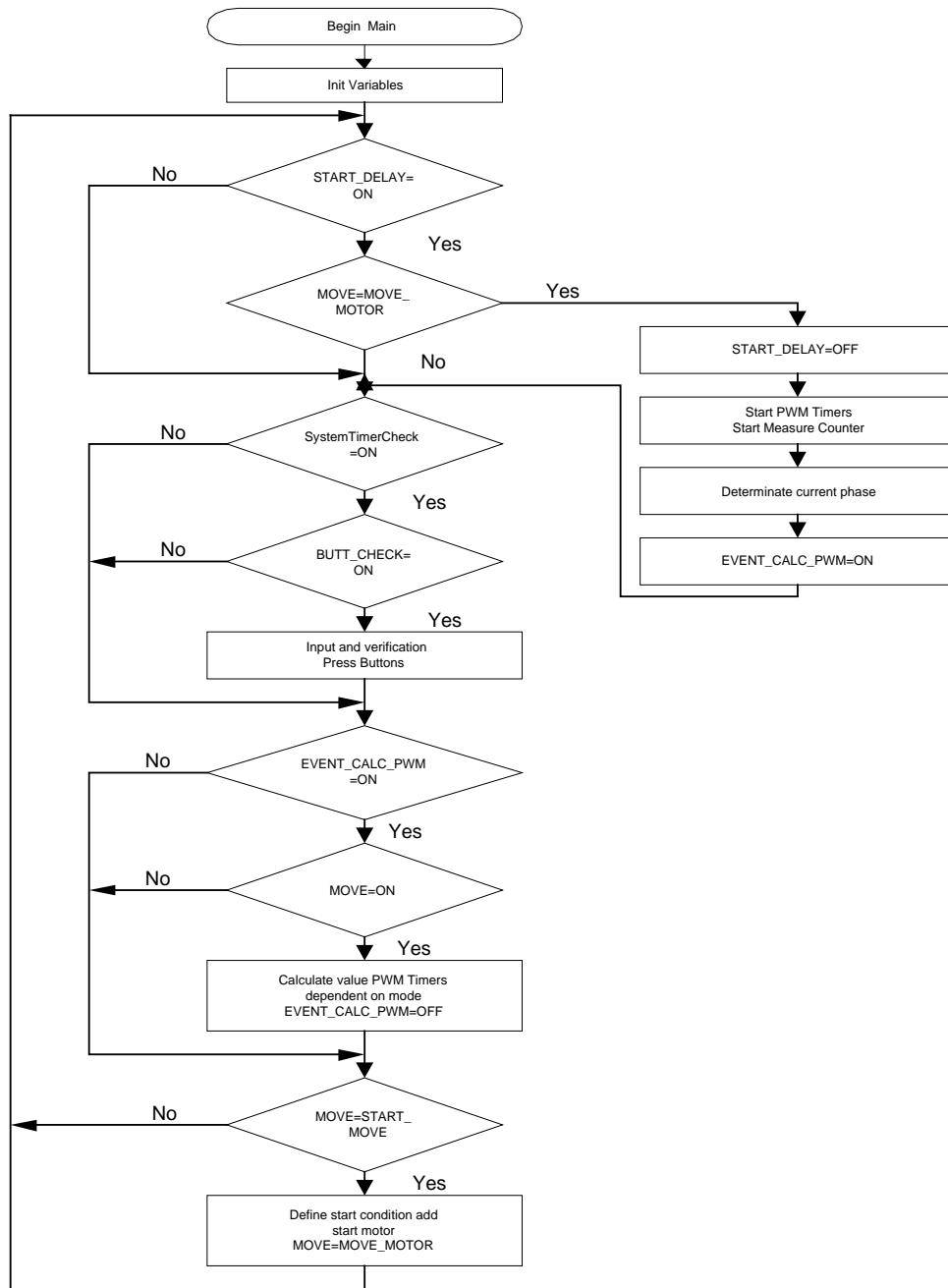
Figure 7. Main Loop Flowchart
