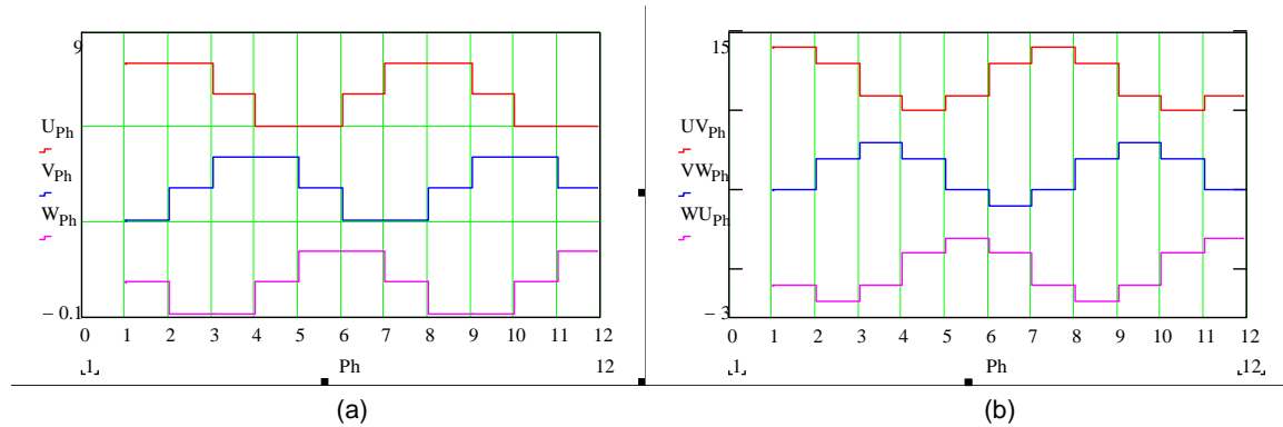
Figure 6. PWM Phase Signals (a) and Motor Winding Voltages (b)
