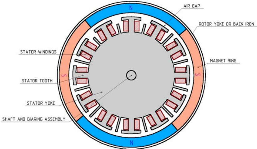
Figure 1. BLDC Motor Internals Outer-Rotor Version
