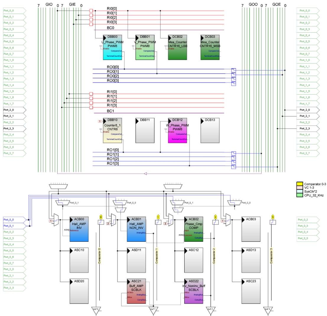
Figure 5. PSoC Internal User Module Placement
