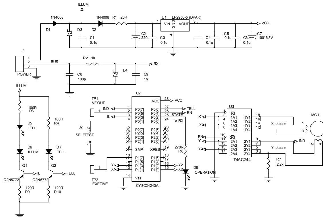
Figure 5. Driver Schematic
