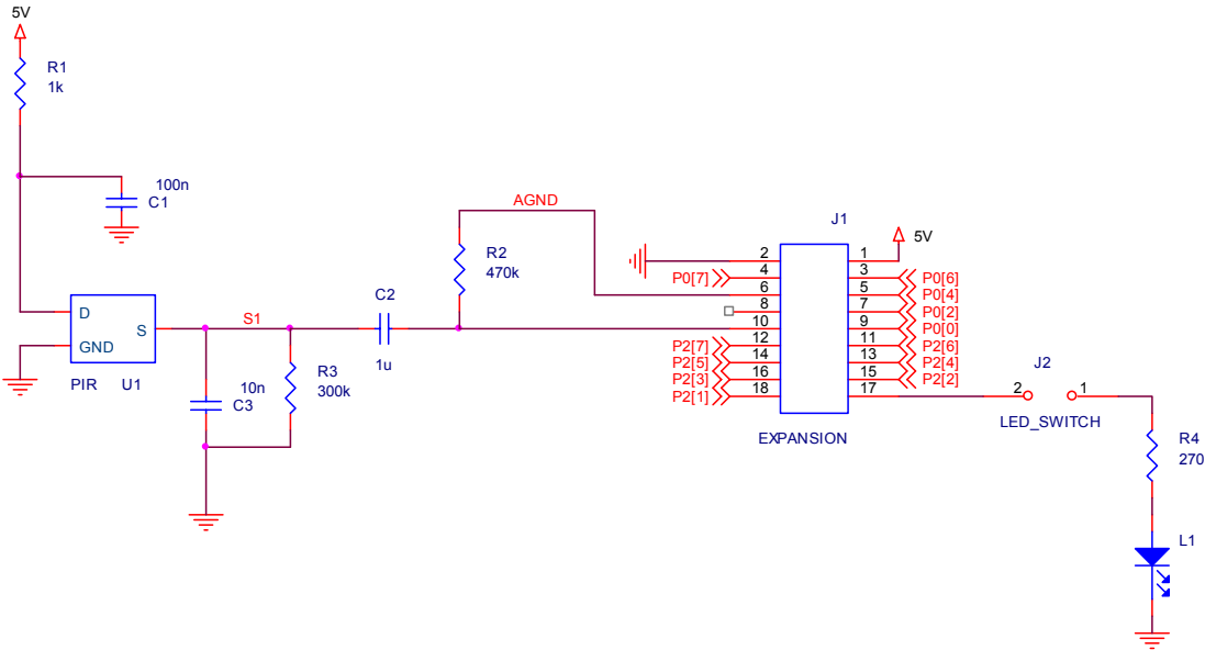
Figure 5. Infrared Motion Sensor Expansion Board Schematic
