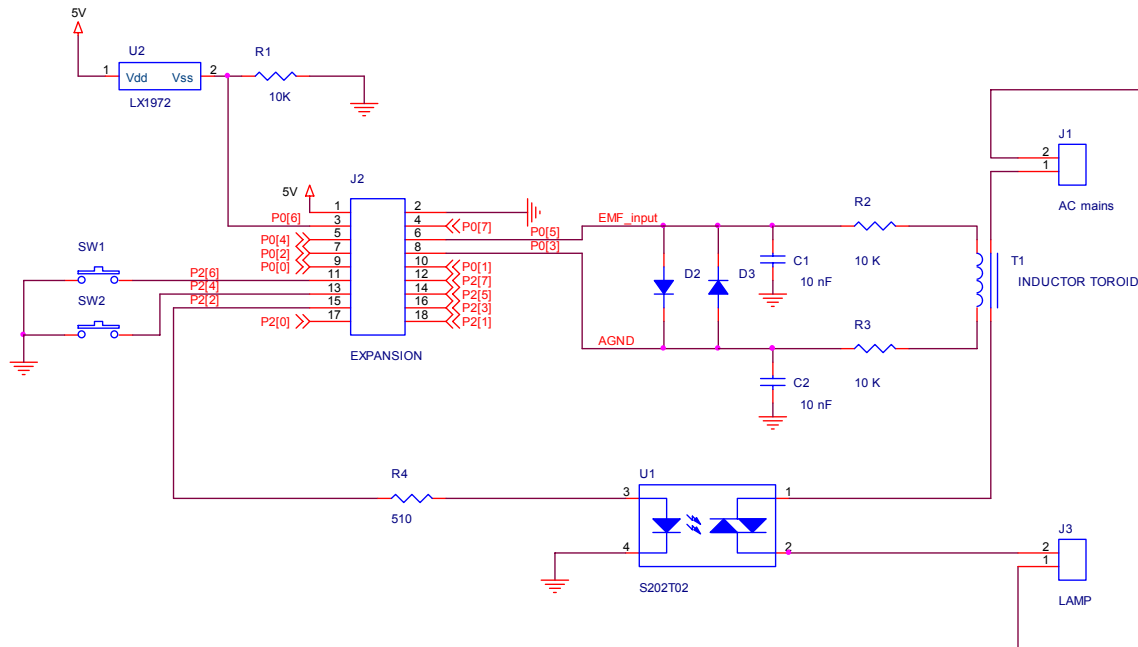
Figure 3. Lighting Control Expansion Board Schematic
