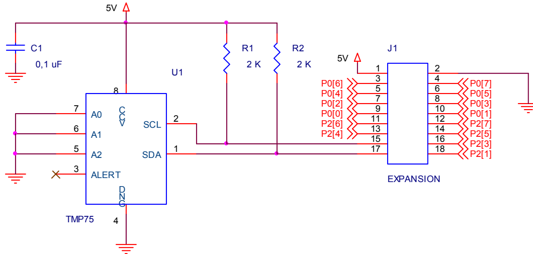
Figure 1. Temperature Sensor Schematic
