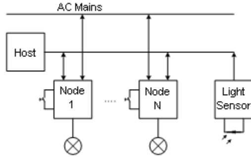
Figure 2. Structure of the Lighting Control Network
